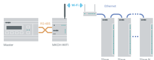
Master в cemu Wi-Fi – Slave в cemu RS-485
